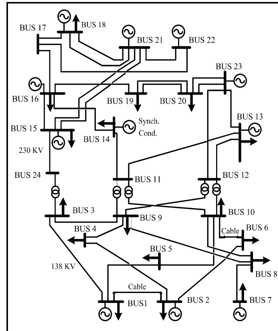
Fig.1. IEEE-RTS system
