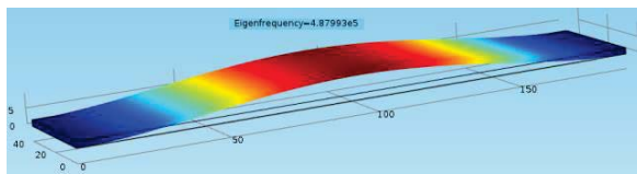
Fig. 4. First mode of resonator (mode1: 490 KHz)
