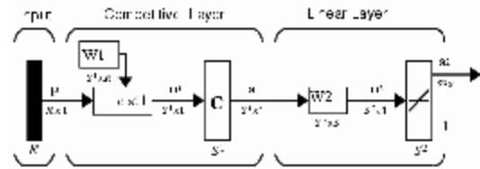
Fig. 2: The LVQ network architecture
