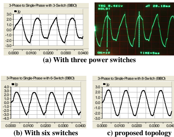
Fig. 8: Output current under balanced operation
