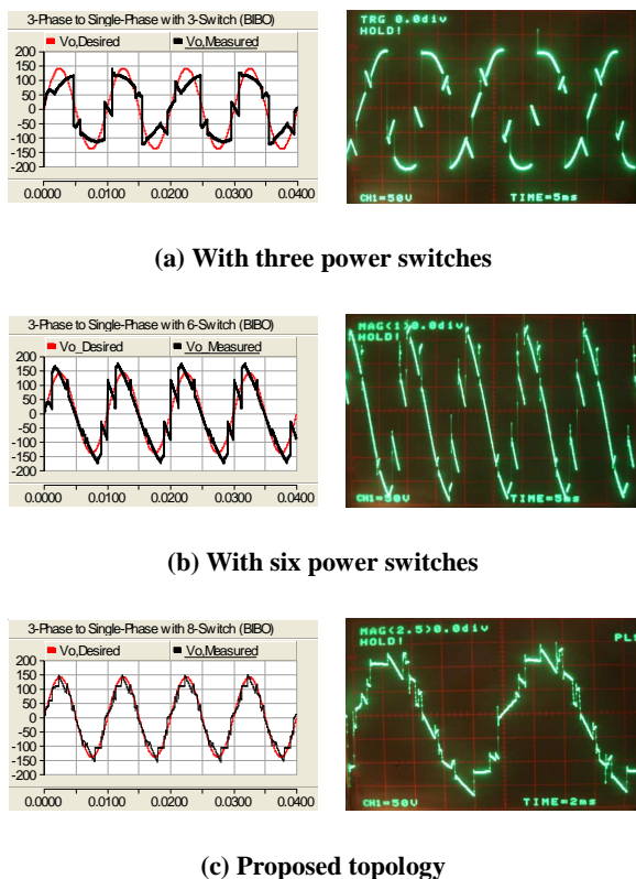
Fig. 7: Output voltage under balanced operation (Left column: Simulation; Right column: Experimental)
