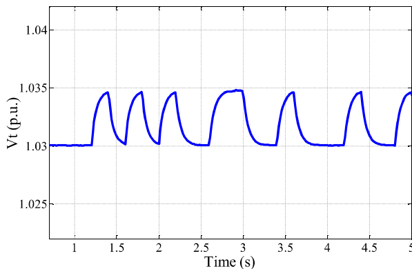
Fig. 5. Terminal voltage
