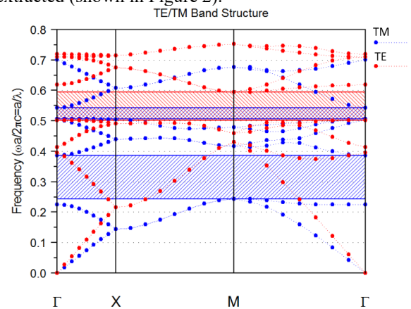
Fig. 2. PBG diagram of the proposed structure.
