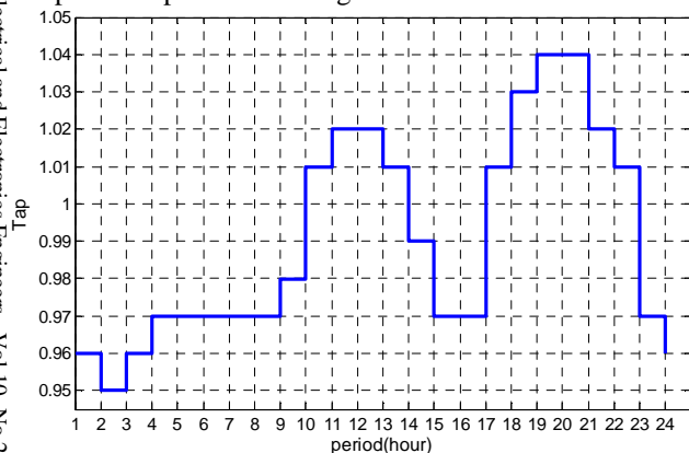
Fig. 12: Tap position based on proposed method
