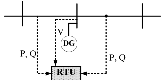
Fig. 5: Details of RTU measurements
