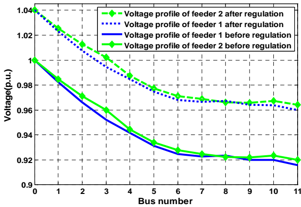
Fig. 16: Voltage profile before and after voltage regulation at 19:00
