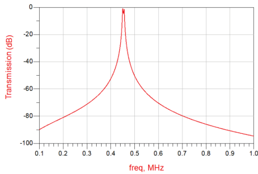
Fig. 8. Frequency characteristic
