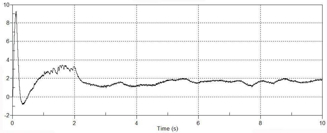
Fig.20. Active power output (MW) - noise component
