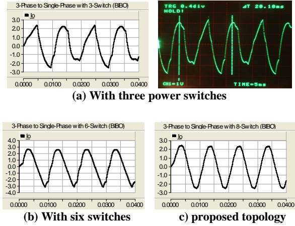
Fig. 8: Output current under balanced operation
