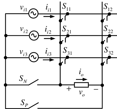
Fig. 3: Proposed topology for three-phase to single-phase matrix converter
