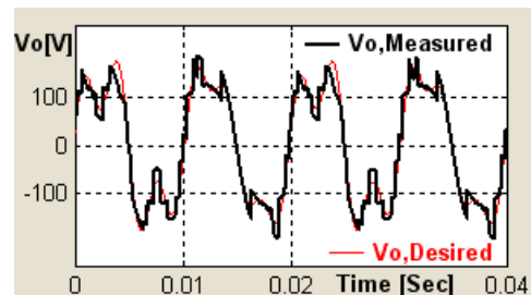
(c) Proposed topology
