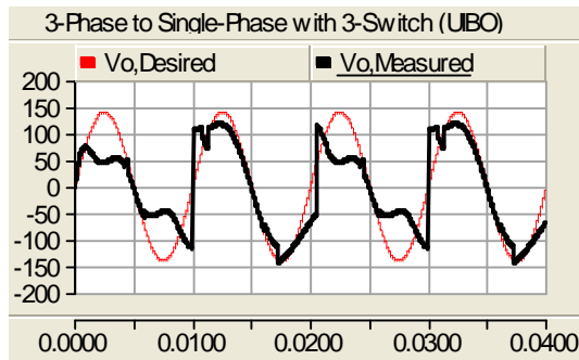
(a) With three power switches
