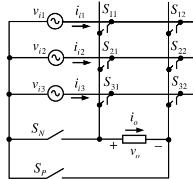
Fig. 3: Proposed topology for three-phase to single-phase matrix converter
