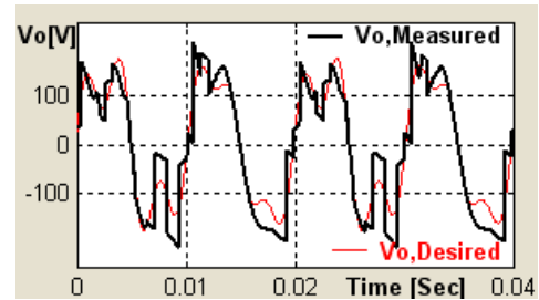
(a) With three power switches
