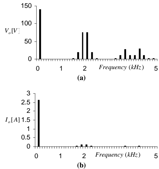
Fig. 16: (a) spectrum of the output voltage, (b) spectrum of the output current
