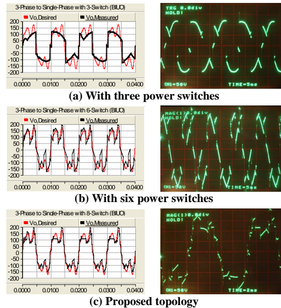
Fig. 11: Output voltage under distorted operation (Left column: Simulation; Right column: Experimental)
