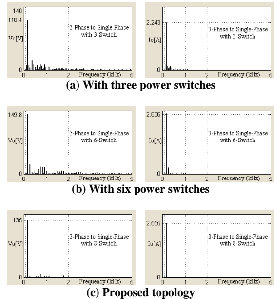
Fig. 9: FFTs of output voltage and current under balanced operation (Left column: Output voltage; Right column: Output current)
