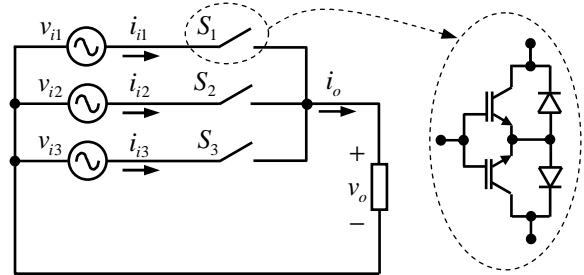
Fig. 1: Three-phase to single-phase matrix converter with three switches
