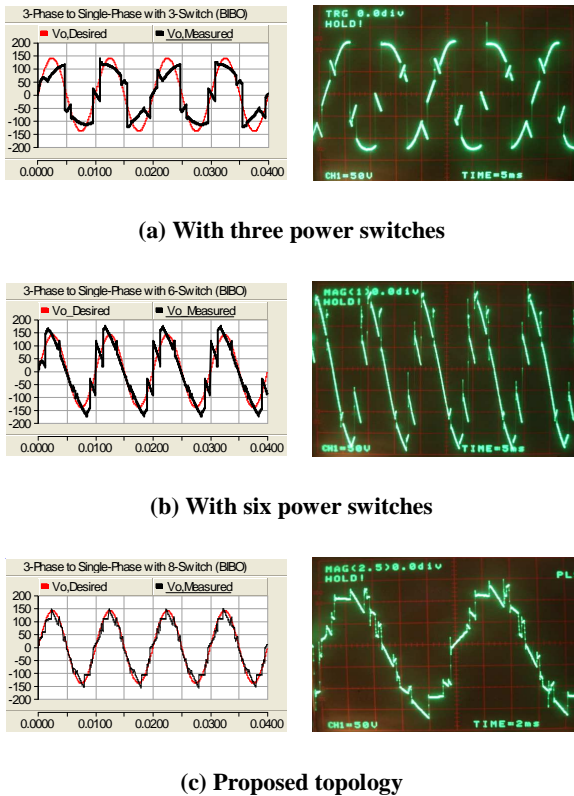
Fig. 7: Output voltage under balanced operation (Left column: Simulation; Right column: Experimental)
