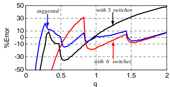
Fig. 5: The percent of voltage error versus voltage transfer ratio
