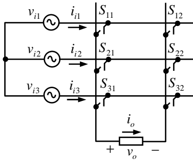
Fig. 2: Three-phase to single-phase matrix converter with six switches
