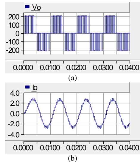
Fig. 15: Simulation results for a three-phase to single-phase ac/dc/ac converter, (a) output voltage, (b) output current
