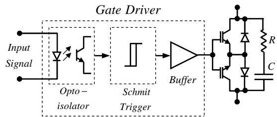
Fig. 6: Gate driver circuit of bidirectional switch
