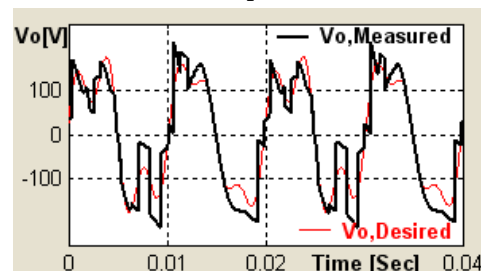
(a) With three power switches
