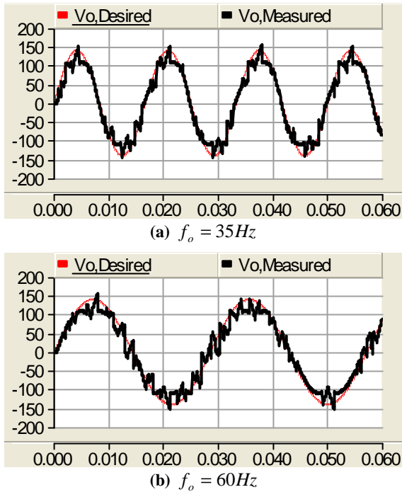
Fig. 14: Output voltage of proposed topology for different output frequencies
