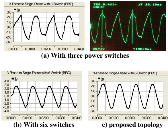
Fig. 8: Output current under balanced operation
