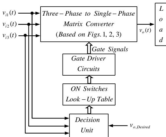
Fig. 4: Block diagram of the proposed control method
