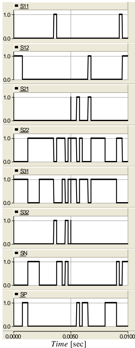
Fig. 10: Commands of switches for the proposed topology
