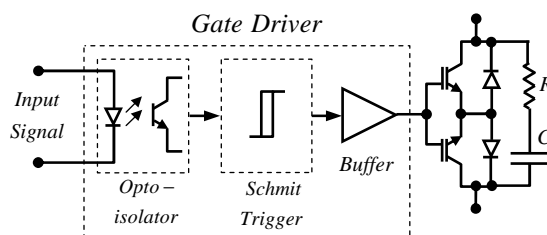
Fig. 6: Gate driver circuit of bidirectional switch
