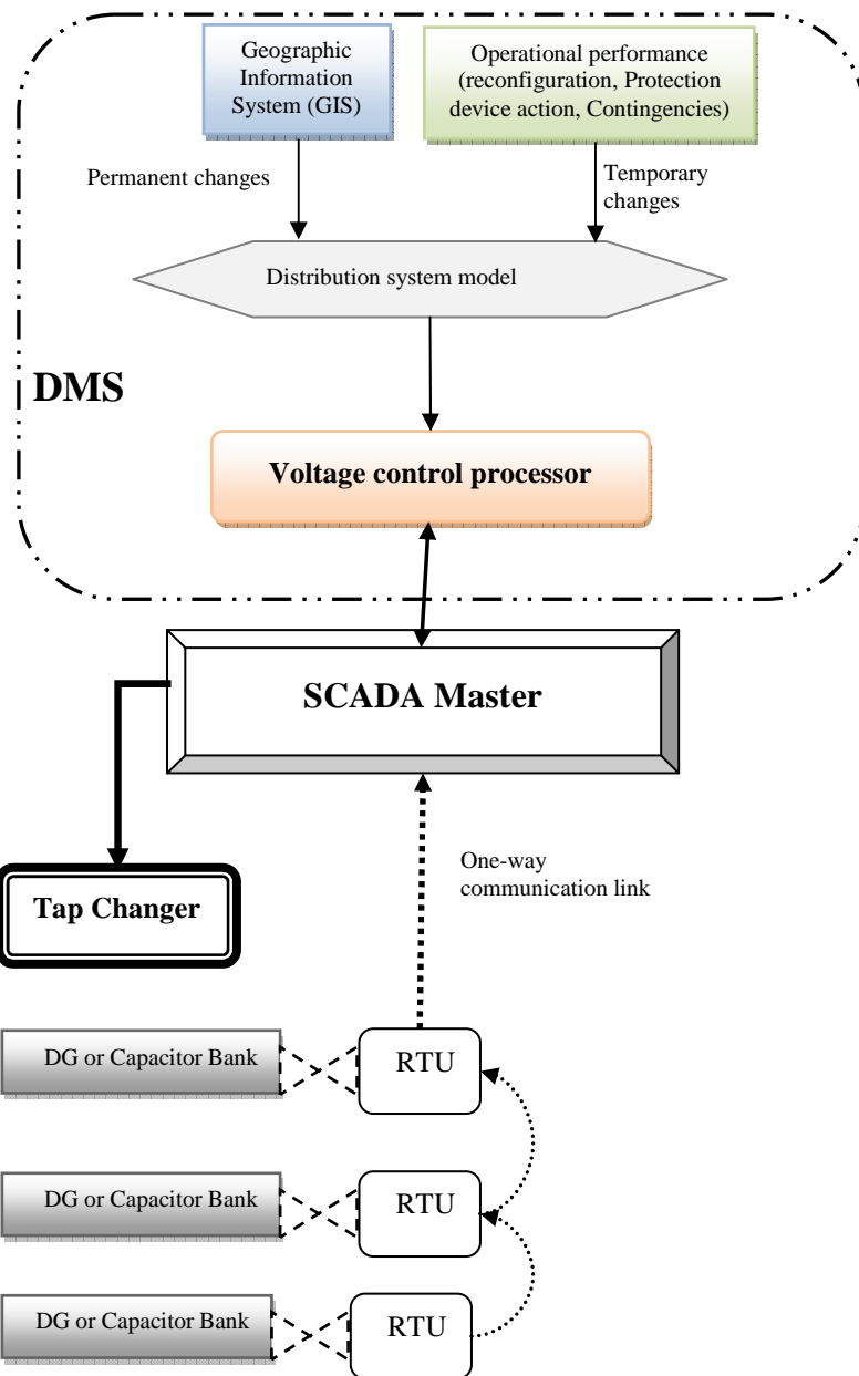
Fig. 3: DMS, SCADA and RTU configuration
