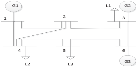
Fig. 2. six-bus system with wind farm
