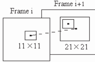
Fig. 3: Cross-correlation based motion tracking
